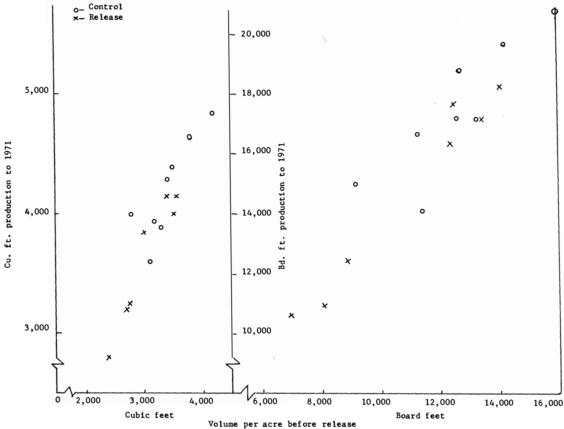
FIGURE 1. Cubic-foot and board-foot production of spruce to 1971 in relation to cubic-foot and board-foot volume per acre of spruce before release.
