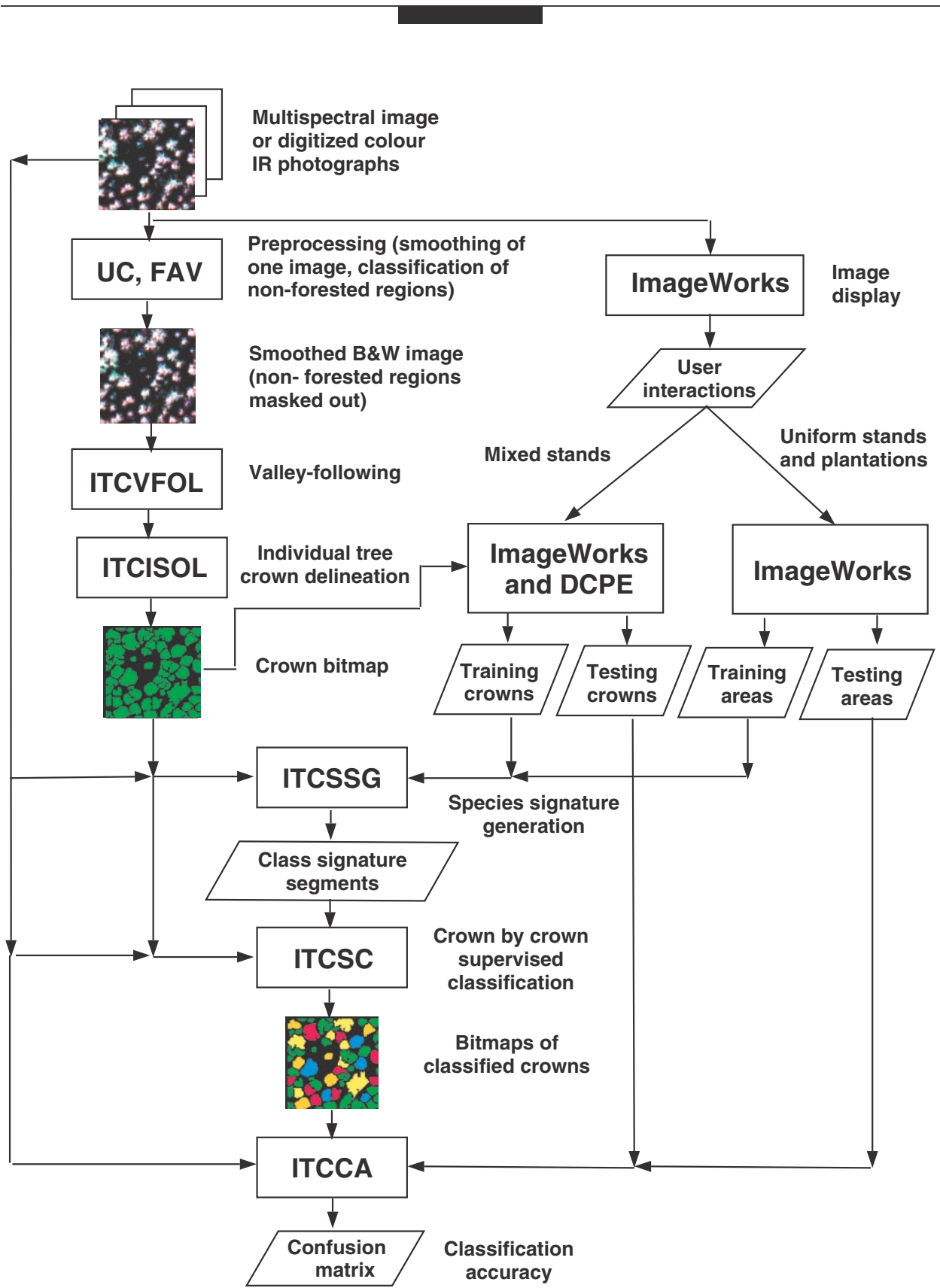
Figure 1 – Methodology for individual tree crown delineation and supervised classification from high spatial resolution multispectral images (from Gougeon 1997).
