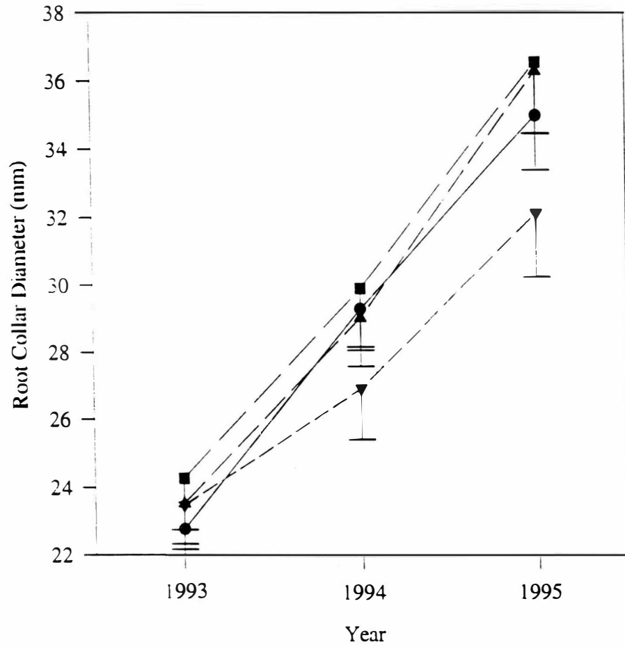
Figure 6 Lodgepole Pine Root Collar Diameter Growth for Block 1 - By Treatment
