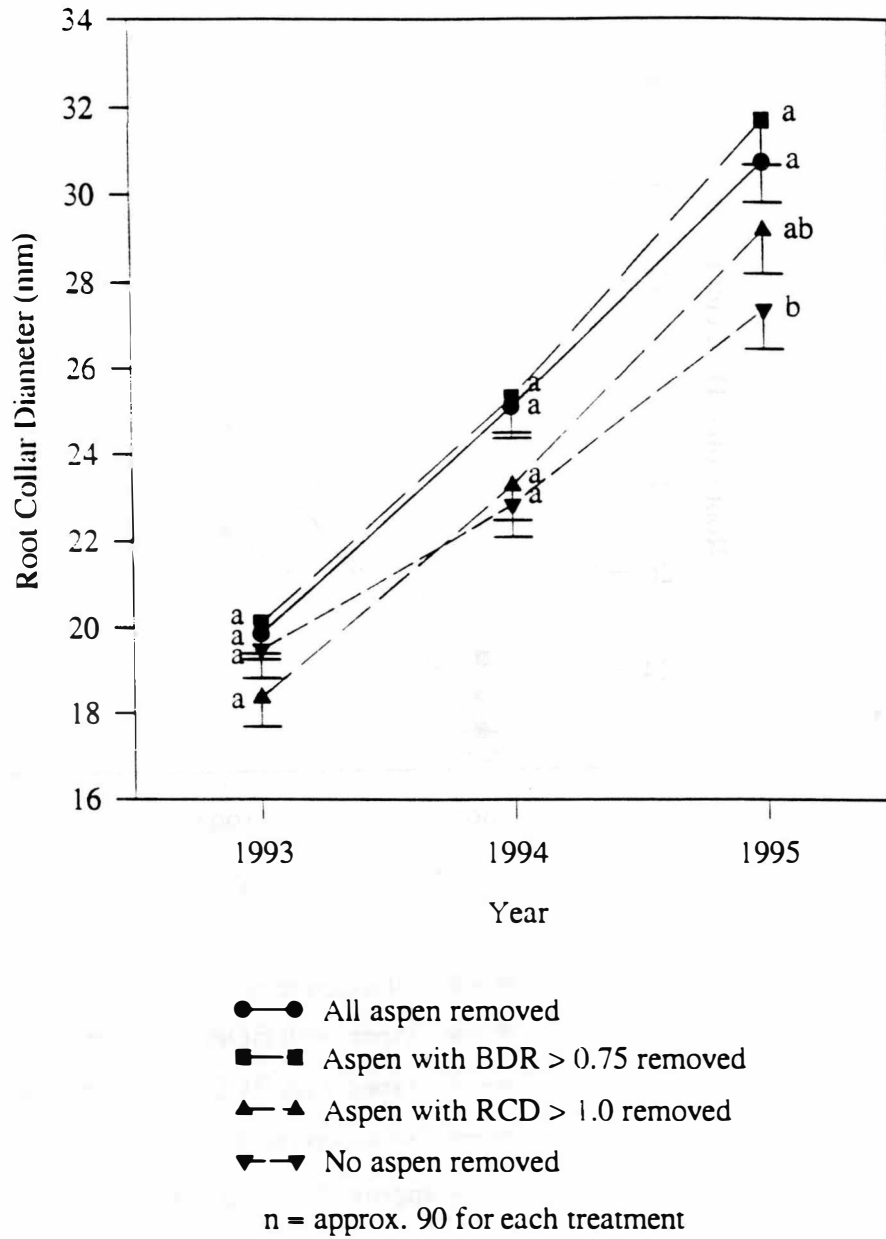
Figure 5 Lodgepole Pine Root Collar Diameter Growth for All Blocks Combined By Treatment
