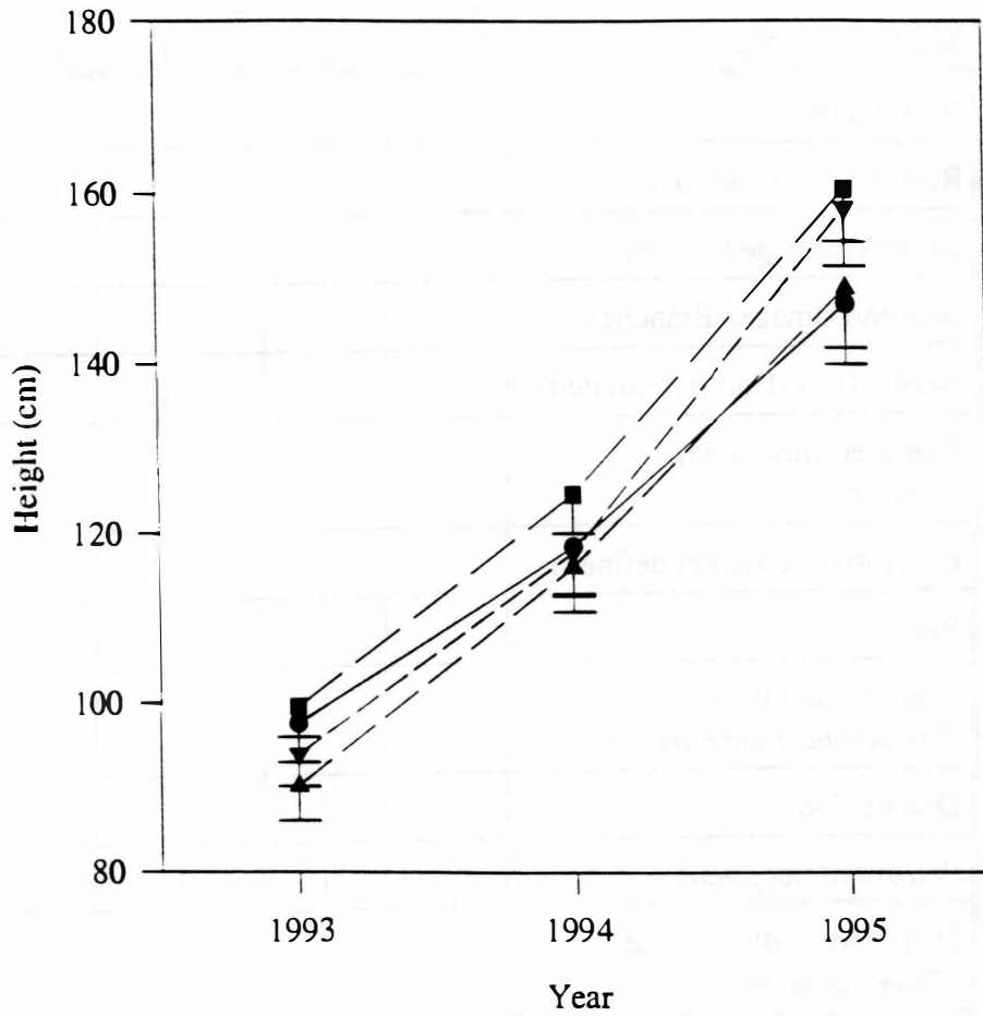
Figure 12 Lodgepole Pine Height Growth for Block 3 - By Treatment
