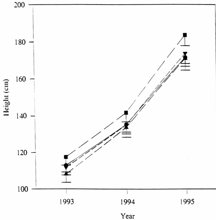
Figure 9 Lodgepole Pine Height Growth for All Blocks Combined - By Treatment
