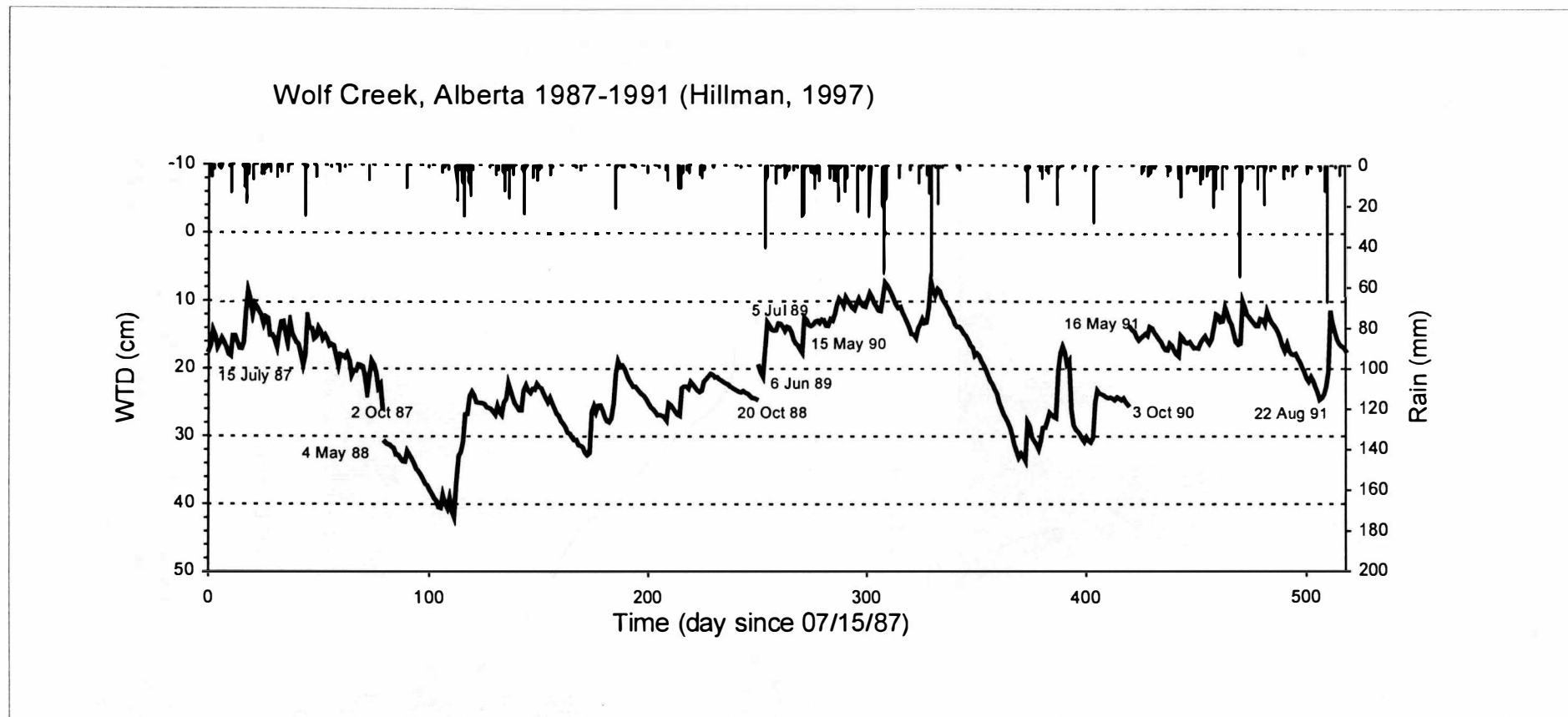
Figure 14. Hydrograph of water-table fluctuations (lower curves) and on-site precipitation (upper bars) at a treed fen site in central Alberta (control #2, Wolf Creek, Alberta) (data from Hillman, 1997). The original measurements were carried out every one and half hours, with total over 7500 readings over five growth seasons (mostly from May to October) from 1987 to 1991. The figure shows the daily variations of WTD and rainfall amount. The normal precipitation (1951-1980) for the region is 536 mm annually, 361 mm of which is during May to September and 150 mm of which are snowfalls. This period has a dry year (1988) with growing season rainfall of 298 mm and a wet year (1990) with growing season rainfall of 423 mm. See text for more discussion.
