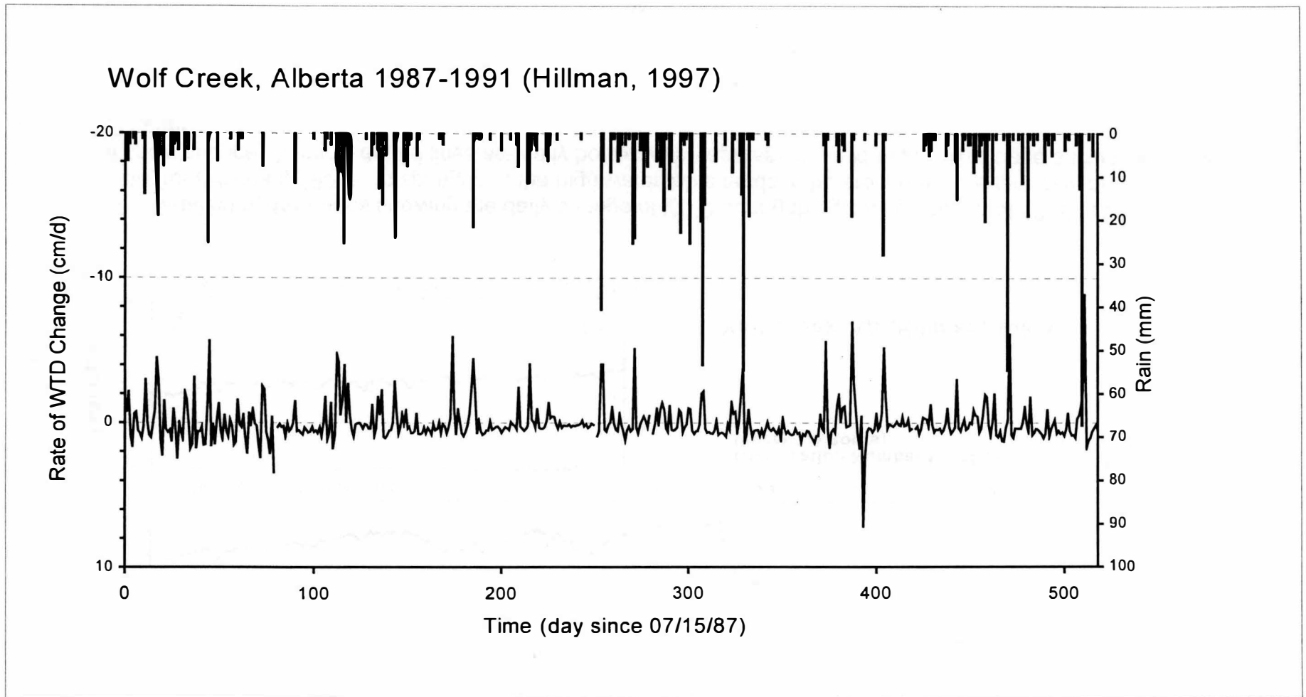
Figure 16. Daily rate of WTD change (curves) in response to rainfall events (bars) at Wolf Creek, Alberta (data from Hillman, 1997).
