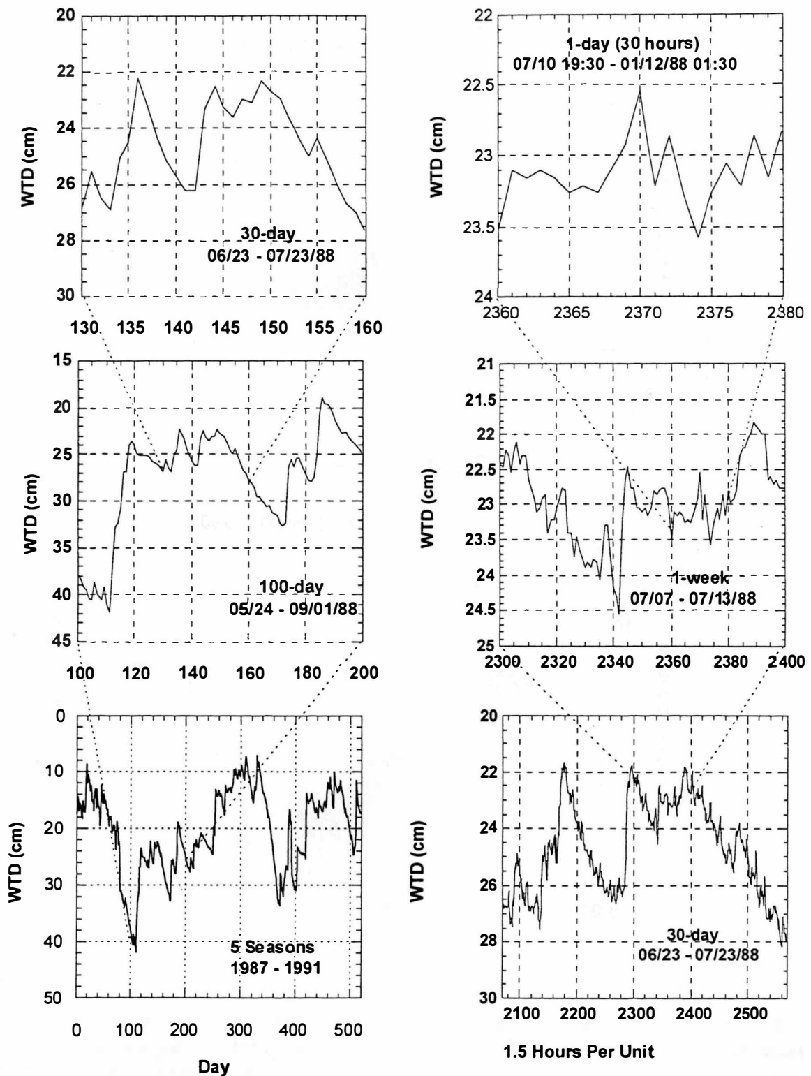
Figure 18. Self-similarity of water-table fluctuations in peatlands at Wolf Creek, Alberta (data from Hillman, 1997). Total record represents growing season (mostly from May to October) for the years 1987-1991.
