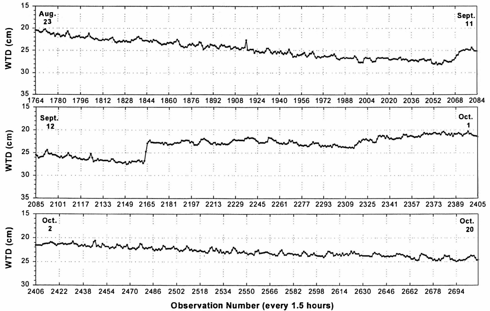
Figure 17. Continued. For autumn from 23 August to 20 October.
