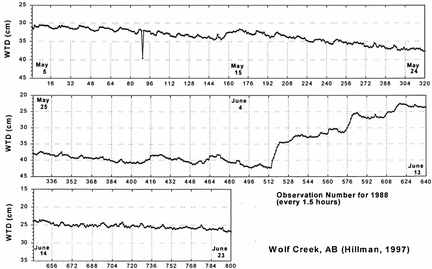
Figure 17. Detailed hydrographs showing the daily change of WTD during the growing season of 1988 at Wolf Creek, Alberta (data from Hillman, 1997). In springtime, the high water table tends to be around noon every day, probably due to melting of snow and ice. Vertical dotted lines are daily boundaries, representing mid-night. This page shows record from 5 May to 23 June.
