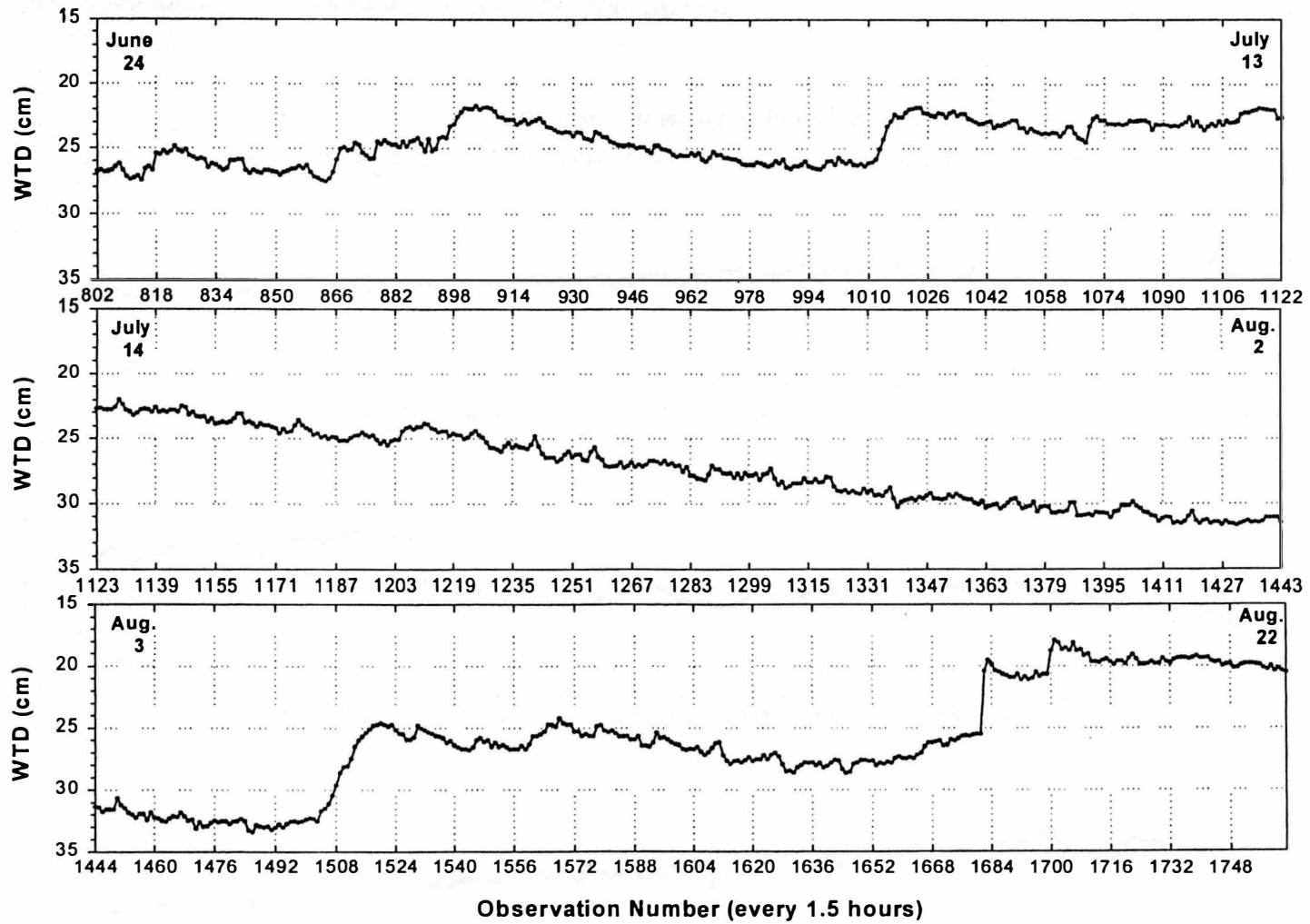
Figure 17. Continued. For summer from 24 June to 22 August.
