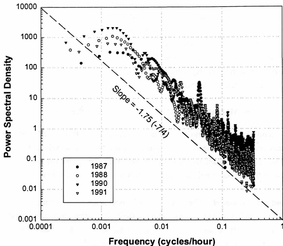
Figure 20. Power spectrum of the WTD time series for 1987, 1988, 1990 and 1991 in a peatland at Wolf Creek, Alberta (data from Hillman, 1997). The power spectrum is given as a function of frequency from time scales of 3 to 3000 hours, as plotted in a log-log scale. The scaling exponent is close to -1.75 ( -7/4 ), suggesting a relation of S(f) \propto 1/f^{-1.75} .
