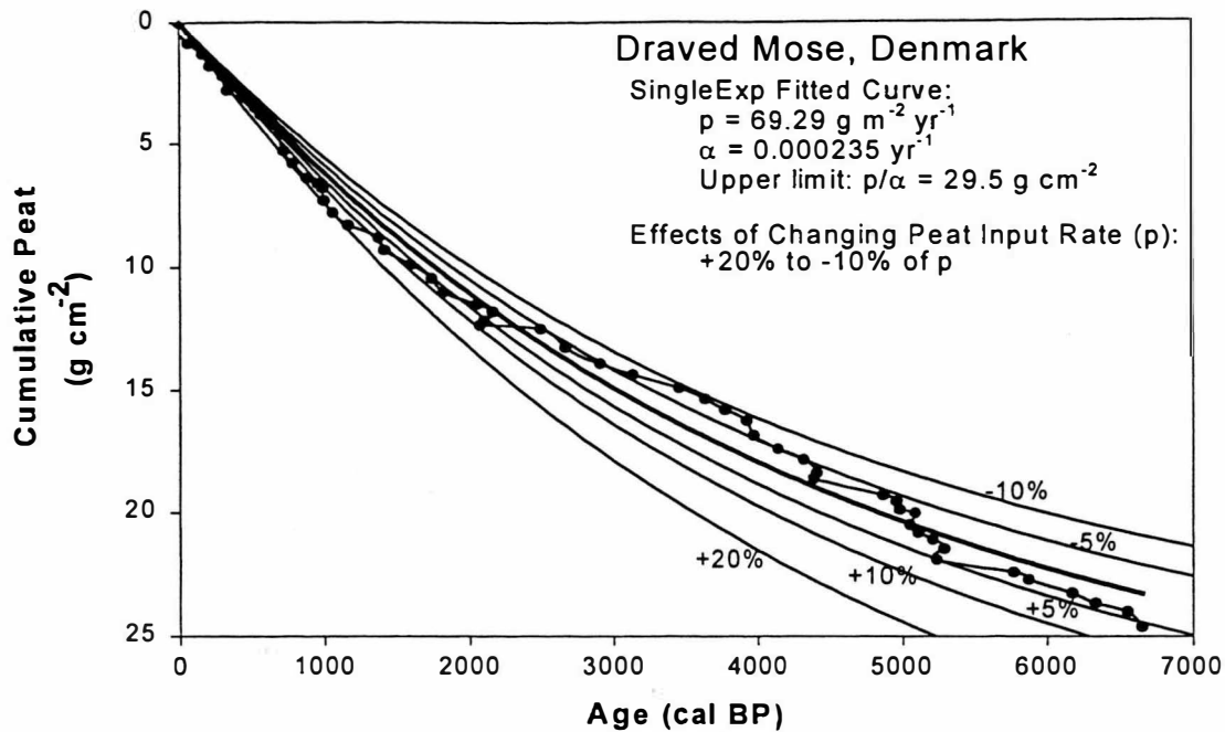
Figure 9. Effects of changing the peat addition rate to the catotelm on the shape of peat mass – age profile, using the Draved Mose peat profile as an example (data from Aaby and Tauber, 1975). Increasing the addition rate causes deeper peat, i.e., the curve moves downward. The central thick curve is fitted by single exponential model.
