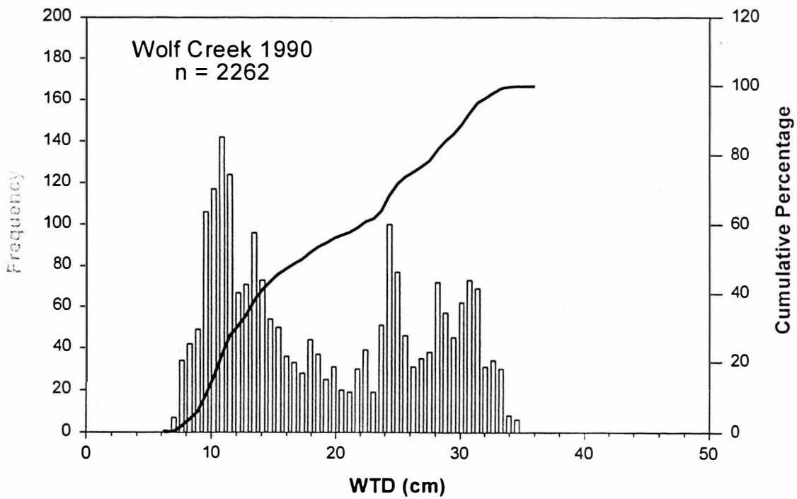
Figure 15. WTD frequency (bars) and cumulative percentage (curves) for 1988 and 1990 at Wolf Creek site (data from Hillman, 1997). In 1988, the WTD is at 22-28 cm for 60% of the time, and in 1990 water level is higher, wider spread but concentrated at 10-15 cm for 40% of the time.
