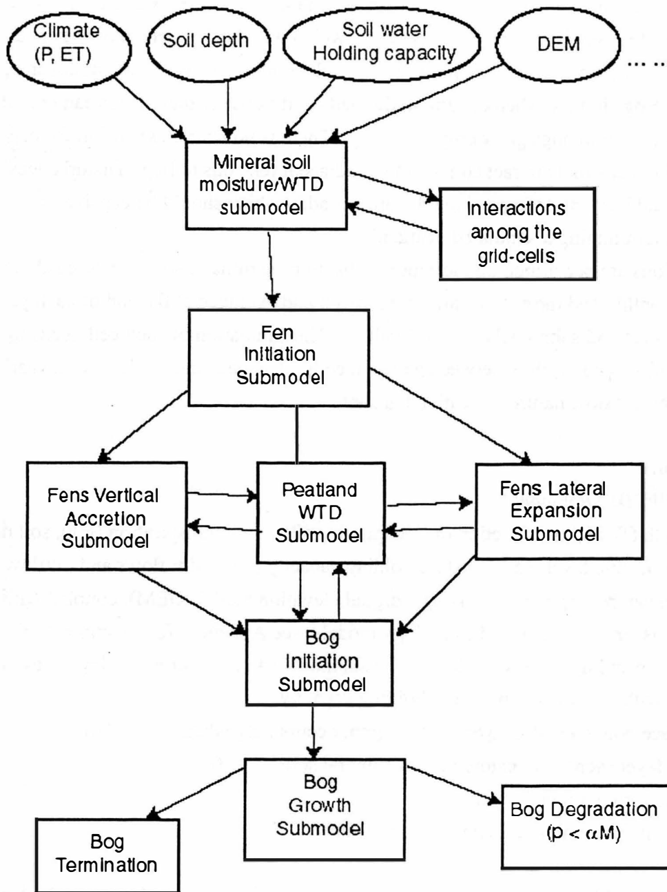
Figure 2. Conceptual design of a 3-D peatland simulation model, which considers peatland initiation, vertical growth and lateral expansion. The model can be dynamically driven by climate variables (e.g., effective moisture).
