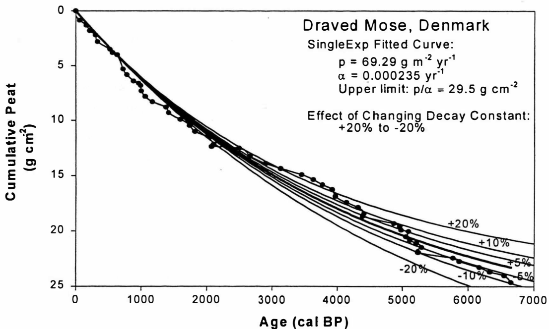
Figure 10. Effects of changing the peat decay rate in the catotelm on the shape of peat mass – age profile, using the Draved Mose peat profile as an example (data from Aaby and Tauber, 1975). Increasing the decay rate causes shallower peat, i.e., the curve moves upward. Compare with Fig. 9, changing addition rate tends to affect both young and old peat, but changing decay rate tends to affect more significantly old peat.
