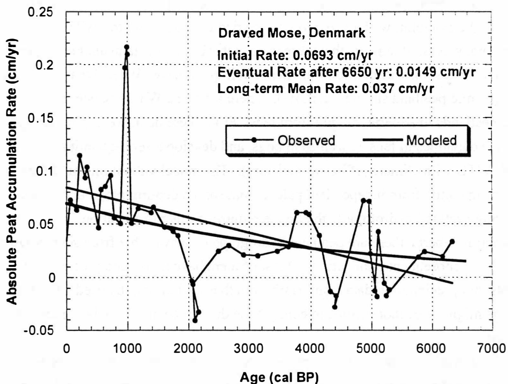
Figure 13. Change of absolute peat accumulation rate over time, using Draved Mose as an example (data from Aaby and Tauber, 1975). The wiggled line is calculated from each pair of dated horizons, the smooth curve is derived from modeled results using a single exponential model, and the straight gray line is a regression line of observed data points. This figure shows that the accumulation rate decreases over time from an initial maximum peat addition rate of 0.069 \text{ cm yr}^{-1} to an eventual rate of 0.015 \text{ cm yr}^{-1} , with a mean of 0.037 \text{ cm yr}^{-1} . The rates are based on the measured smooth curve.
