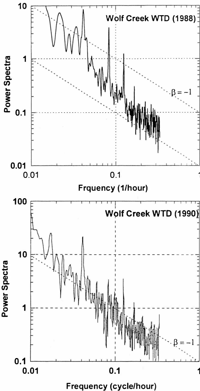
Figure 19. Power spectrum of the WTD time series for 1988 and 1990 in a peatland at Wolf Creek, Alberta (data from Hillman, 1997). The power spectrum is given as a function of frequency from time scales of 3 to 100 hours, as plotted on a log-log scale. The scaling exponent is about -1.4 and -1.2 for 1988 and 1990, respectively, suggesting a relation of S(f) \propto 1/f^{-1.4} and S(f) \propto 1/f^{-1.2} . The power-law behavior of peatland WTD dynamics may suggest the presence of fractal-like, self-regulating mechanisms in peatlands.
