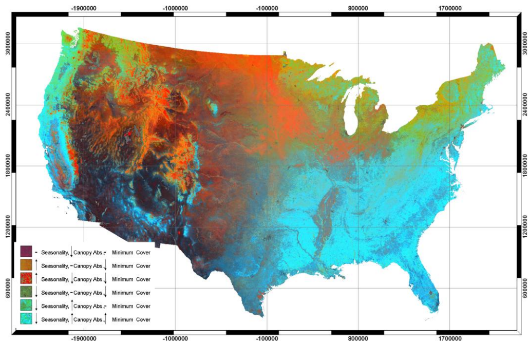
Figure 2: The combined dynamic habitat index derived from 2000 – 2005. Ecoregion boundaries are highlighted in grey. The image was derived by assigning annual integrated greenness to the green band, minimum cover to the blue band, and seasonality to the red band. Bright red areas, which have low annual mean fPAR (the fraction of absorbed photosynthetically active radiation), low annual minimum fPAR and high seasonal variability, indicate locations with only a small amount of primary production evident for part of the year. Bright cyan areas have a high mean, a high minimum and low variability and represent locations with vegetation that was consistently productive throughout the year. Darker blue indicates landscapes with a low mean, a high minimum, and low variability. Orange areas indicate moderately productive vegetation that varied in productivity throughout the year. Green areas represent high annual production, a high annual minimum production and low seasonality. Symbols: ↑High, ↓Low and –moderate.
