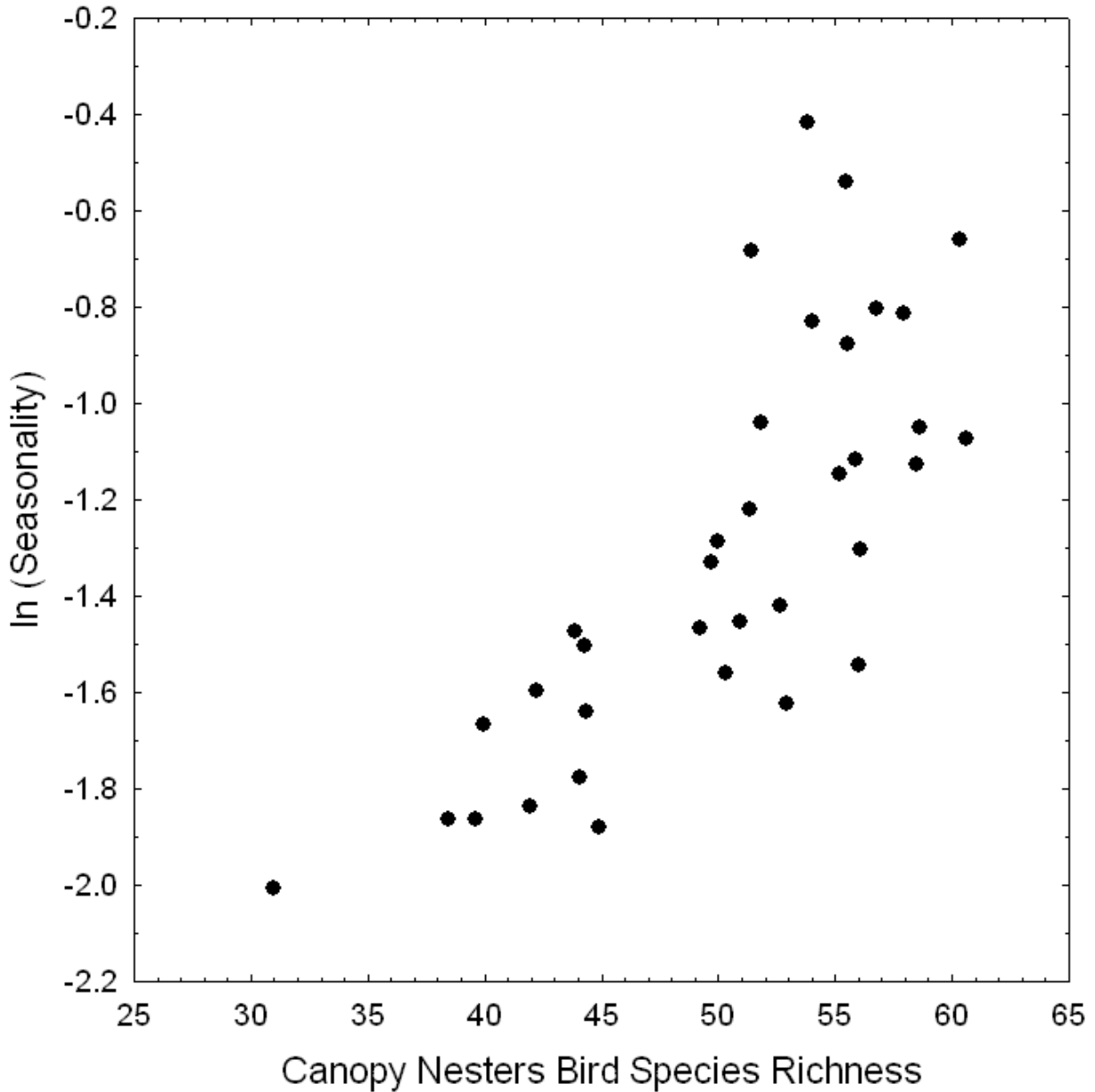
Figure 5. Scatter plots showing relationship between (a) grassland breeding bird species richness and seasonality (using a natural logarithm transformation) over all ecoregions regardless of land cover type, and (b) canopy nesting bird species richness and seasonality (using a logarithm transformation) for forest dominated ecoregions. Correlations and significance for each relationship are shown in Table 1.
