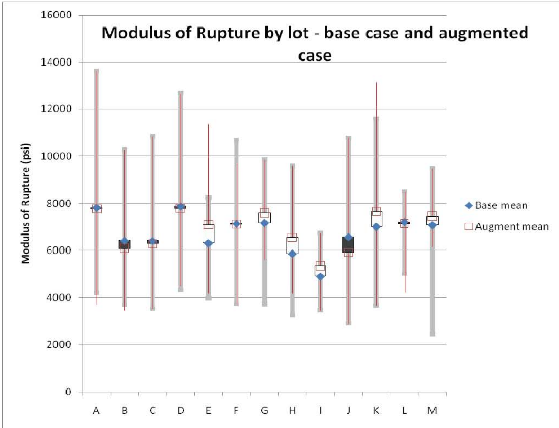
Figure 2. Modulus of Rupture by Lot
