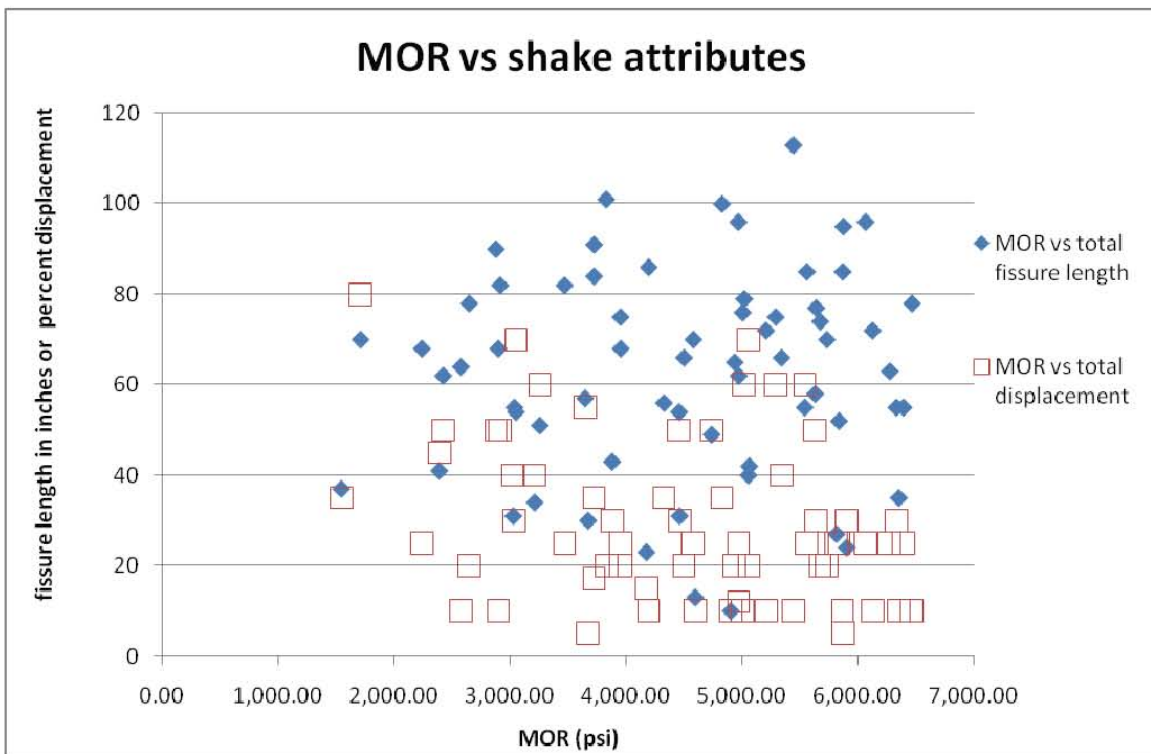
Figure 1. Modulus of Rupture versus shake attributes
