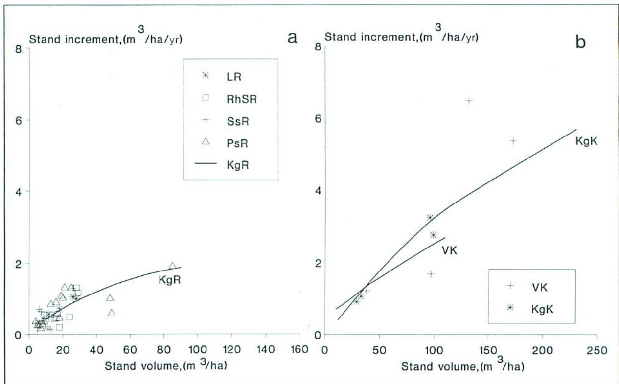
Figure 2. MAI over the past 5 years as a function of stand volume on (a) undrained pine mires and (b) undrained hardwood-spruce mires in northern Finland. Plotted observations indicate the SINKA stands (see text); curves were derived from data in Gustavsen and Päivänen (1986)
