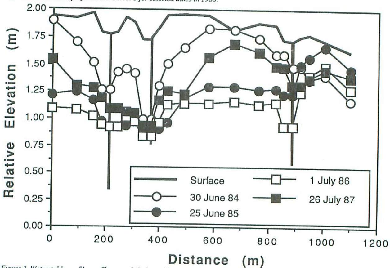
Figure 3. Water-table profiles on Transect 1 during midsummer, 1984-1987.
