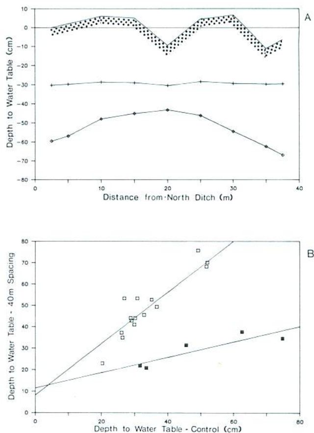
Figure 2. Goose River, 1986-1988, 40-m spacing. Depth to mineral soil is 96 cm. A) Average water-table profiles before (+) and after (◆) drainage. B) Regression lines before (■) [ y = 0.36x + 11.54, r^2 = 0.79 ] and after (□) [ y = 1.20x + 8.36, r^2 = 0.87 ] drainage.
