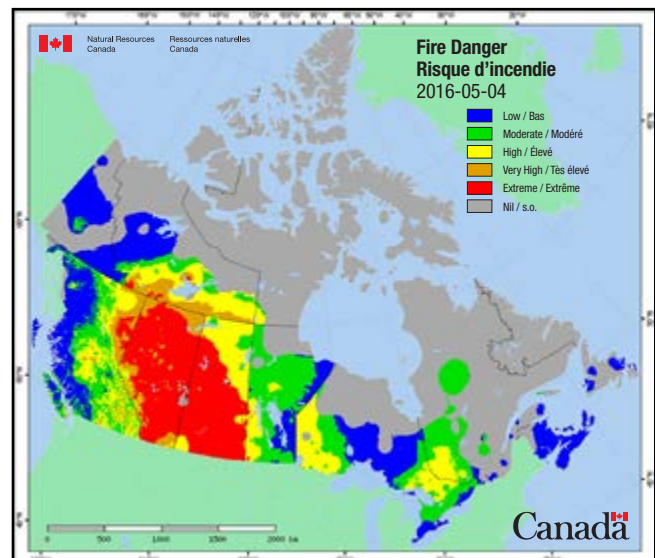
Fire danger forecast for May 4, 2016, Canadian Wildland Fire Information System.
