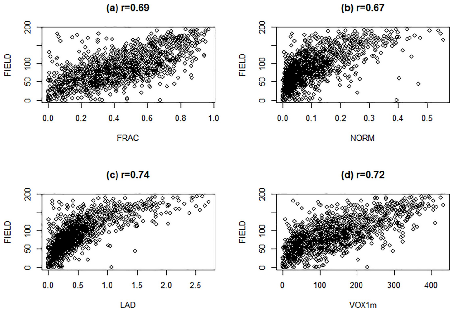
Fig 2. Scatterplot of FIELD (measured density) against the LiDAR metrics, a) fractional cover (FRAC), b) normalized cover (NORM), c) leaf area density (LAD), and d) voxel cover (VOX1m), including Pearson product-moment correlation coefficients.
